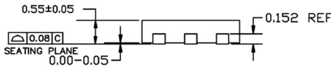
END VIEW NOTE: 1, 2, 3
