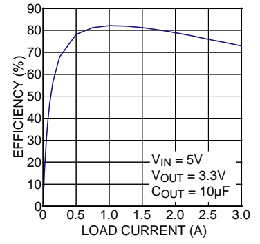
MIC38300 Efficiency
