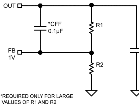
Figure 1. Adjustable Regulator with Resistors
