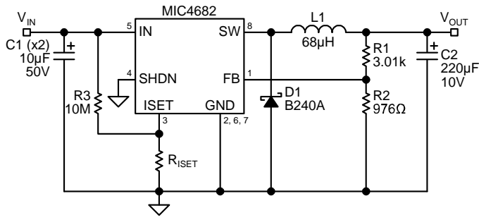
Current Limit Test Circuit
