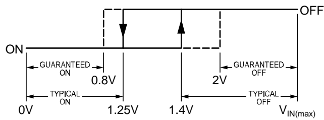
Shutdown Hysteresis
