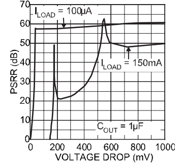
PSRR vs. Voltage Drop
