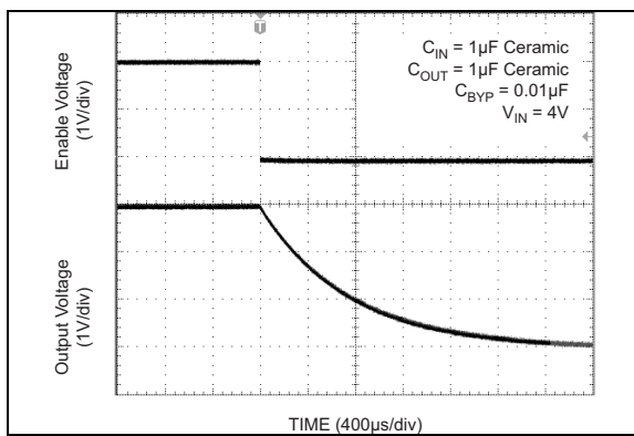
FIGURE 2-20: Shutdown Delay.
