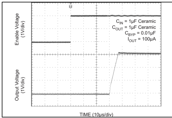
FIGURE 2-19: Enable Pin Delay.
