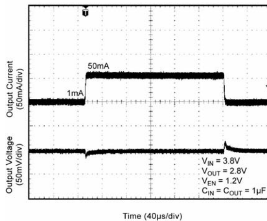
Load Transient
