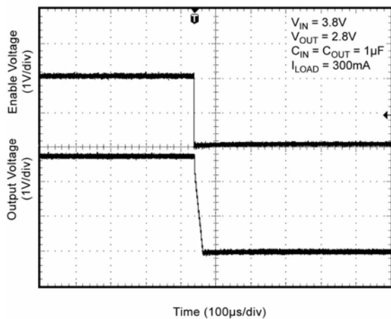
Turn-Off Time
