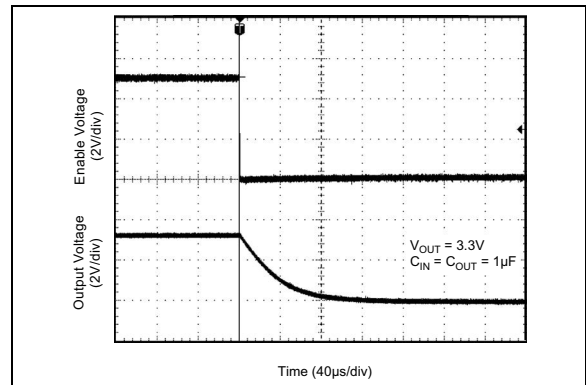
FIGURE 2-17: MIC5368 Auto-Discharge (No Load).
