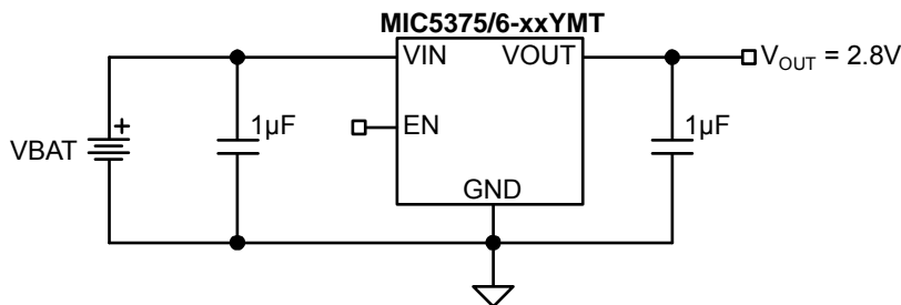
Typical Application
