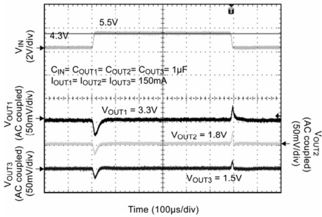
Line Transient
