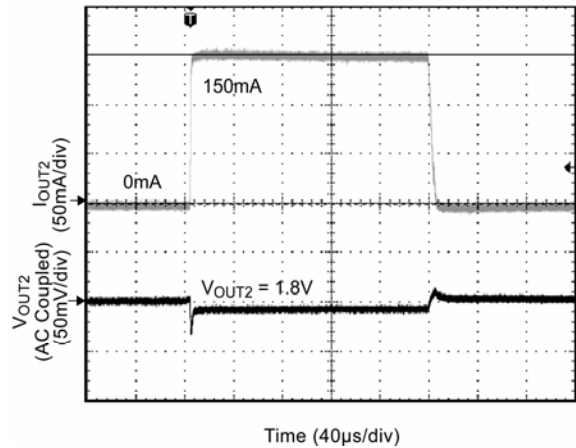
Load Transient VOUT2 (IOUT2 = 0mA to 150mA)
