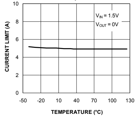
Short Circuit Current vs. Temperature
