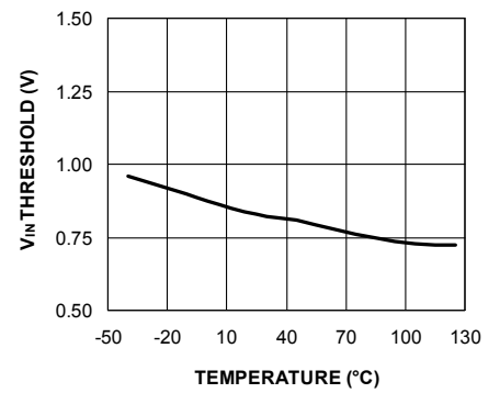
V IN Turn-On Threshold vs. Temperature
