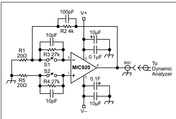
FIGURE 3-2: Noise Measurement.
