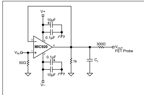
FIGURE 3-4: Closed Loop Frequency Response Measurement.
