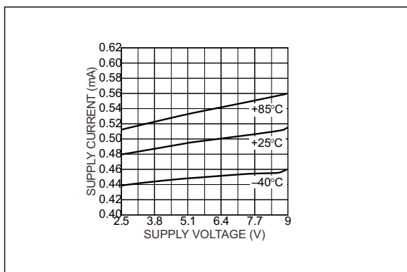
FIGURE 2-3: Supply Current vs. Supply Voltage.
