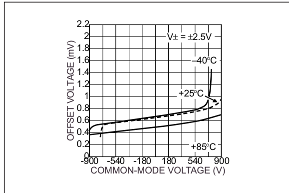
FIGURE 2-4: Offset Voltage vs. Common-Mode Voltage.
