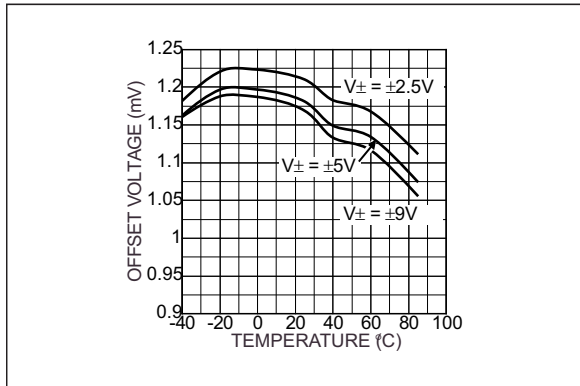
FIGURE 2-1: Offset Voltage vs. Temperature.
