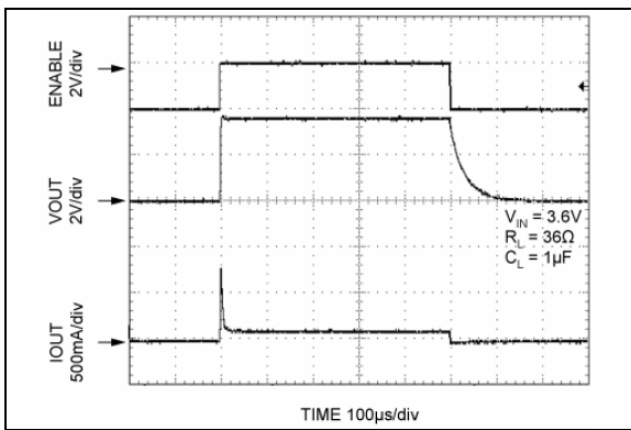
FIGURE 2-18: Turn-On/Turn-Off Timing.
