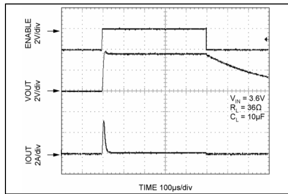
FIGURE 2-20: Turn-On/Turn-Off Timing.
