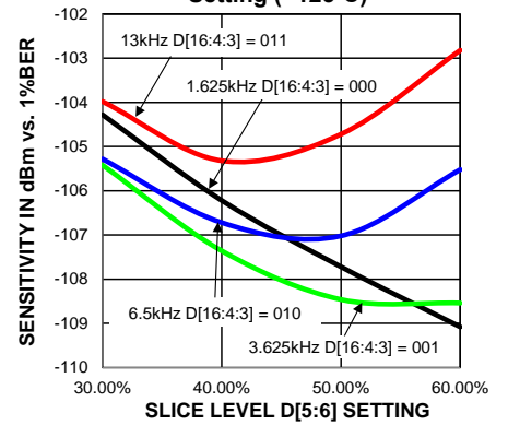
Sensitivity in 433.92MHz vs. Slice Level at Different BW Setting (+125°C)
