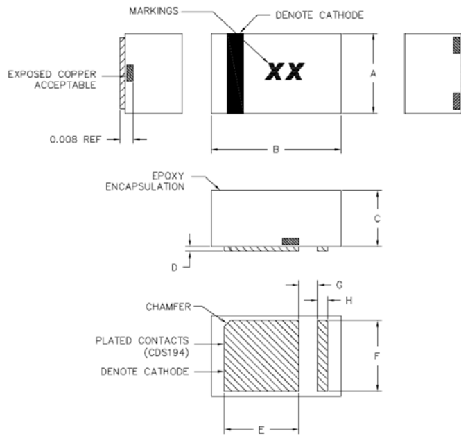
Figure 4 Package Outline
