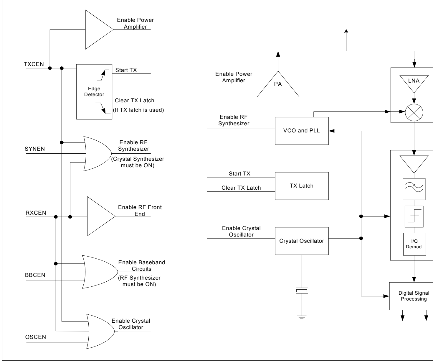
FIGURE 3-12: LOGIC CONNECTIONS BETWEEN POWER CONTROL BITS
