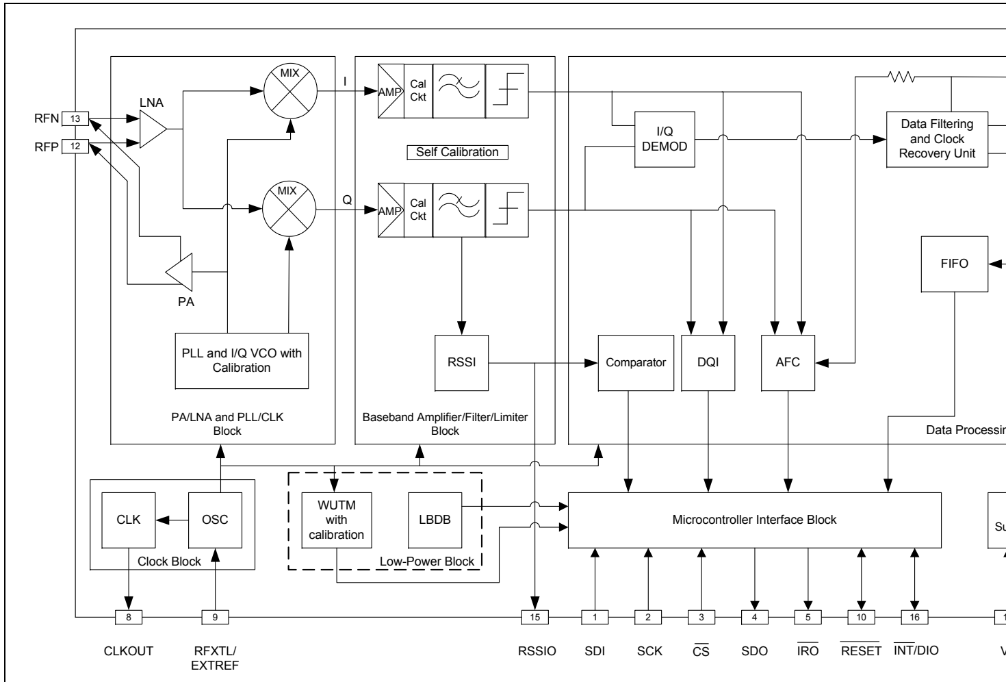
FIGURE 2-1: MRF49XA ARCHITECTURAL BLOCK DIAGRAM
