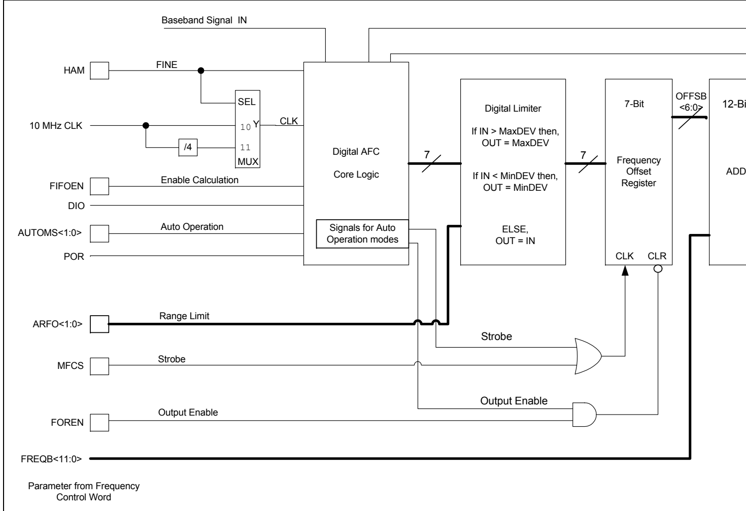
FIGURE 3-6: AFC CIRCUIT FOR FREQUENCY OFFSET CORRECTION
