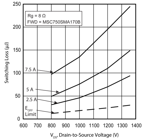
Figure 12 • Switching Energy vs. V_{DS} & I_D
