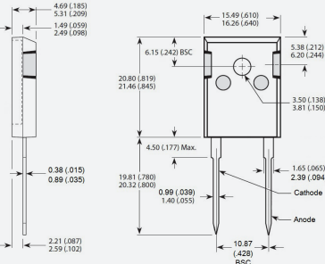
TO-247 2-Lead
