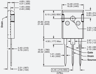
TO-247 3-Lead
