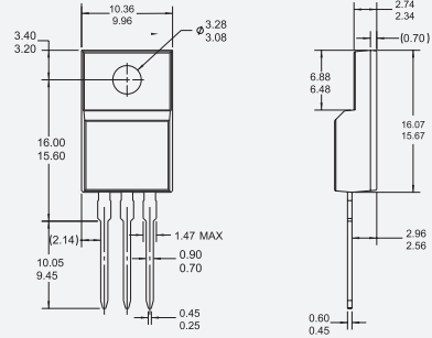
TO-220 [KF]
