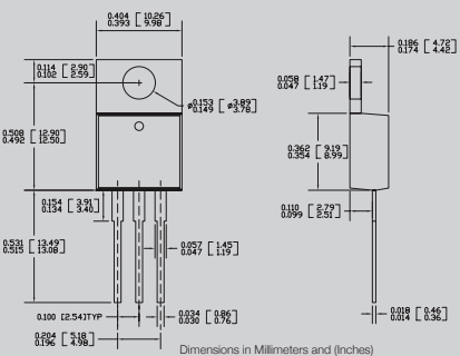
TO-220 3-Lead
