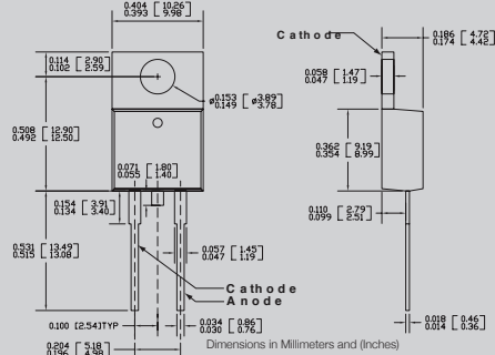
TO-220 2-Lead
