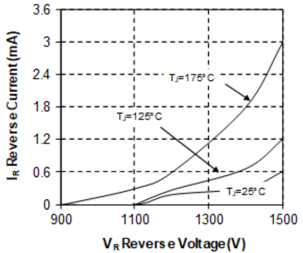
Figure 18 • Reverse Characteristics
