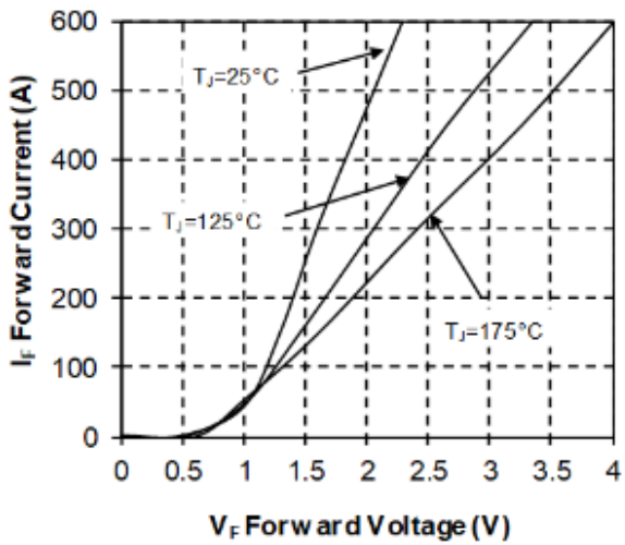
Figure 17 • Forward Characteristics
