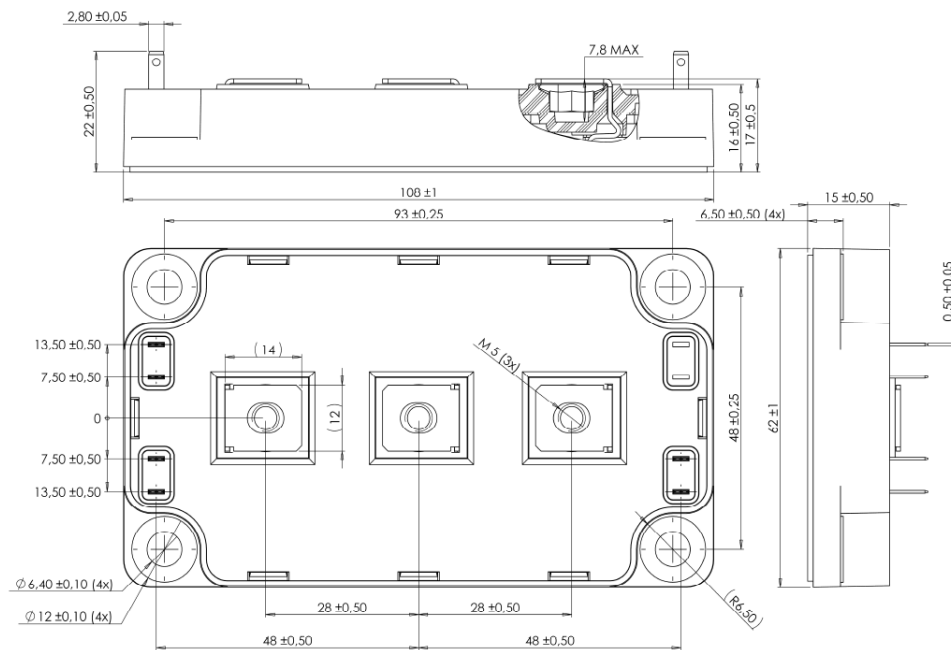
Figure 20 • Package Outline
