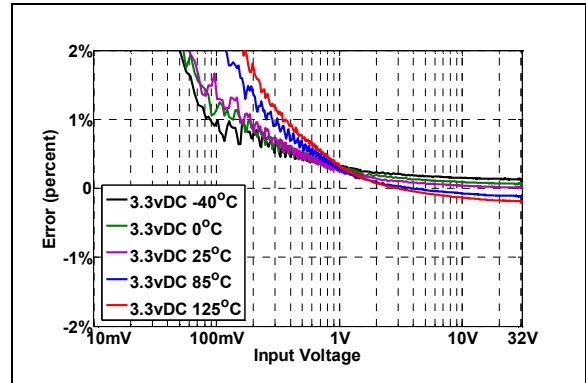
FIGURE 2-11: V_{BUS} Error vs. V_{BUS} Input Voltage vs. Temperature (Zoom View).
