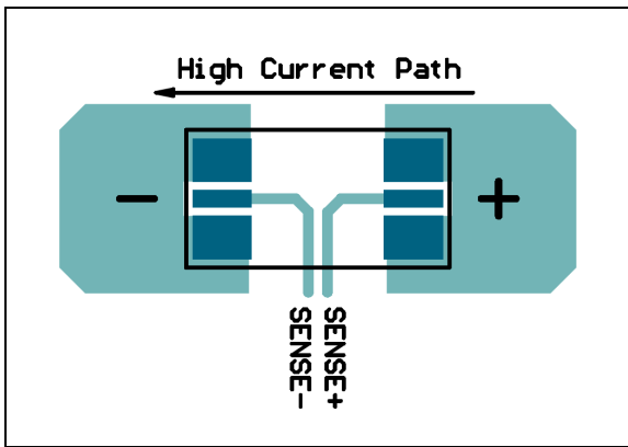
FIGURE 4-3: PCB Pattern for Sense Resistor.
