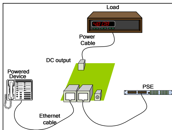
Figure 6: Test Setup
