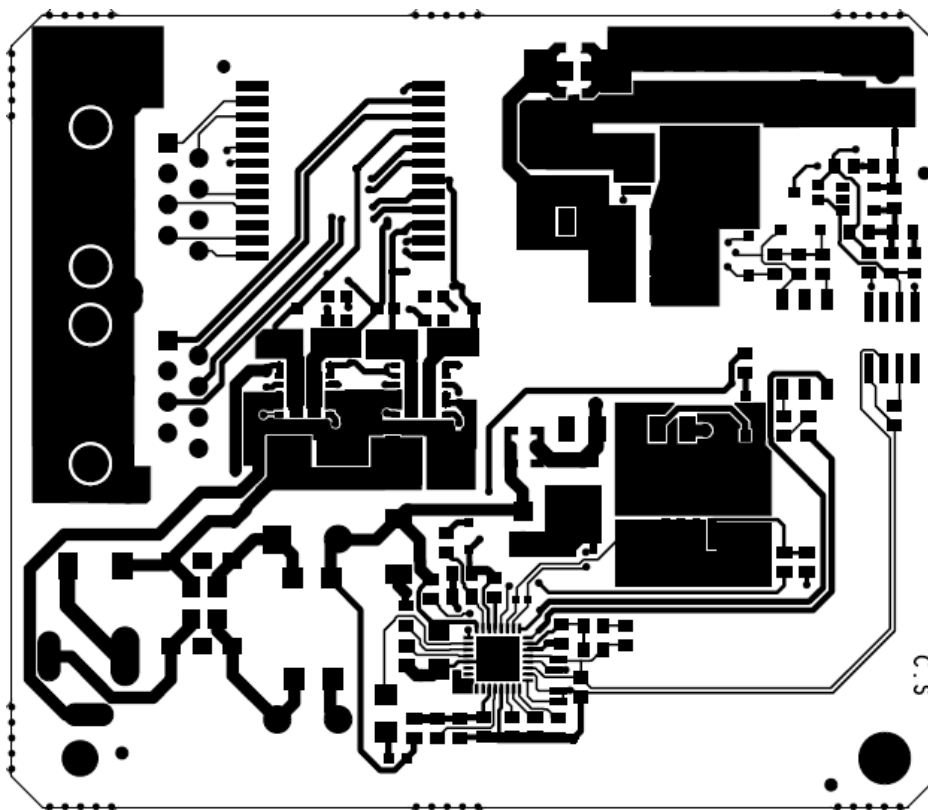
Figure 27: Top Layer
