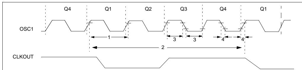
FIGURE 17-5: EXTERNAL CLOCK TIMING
