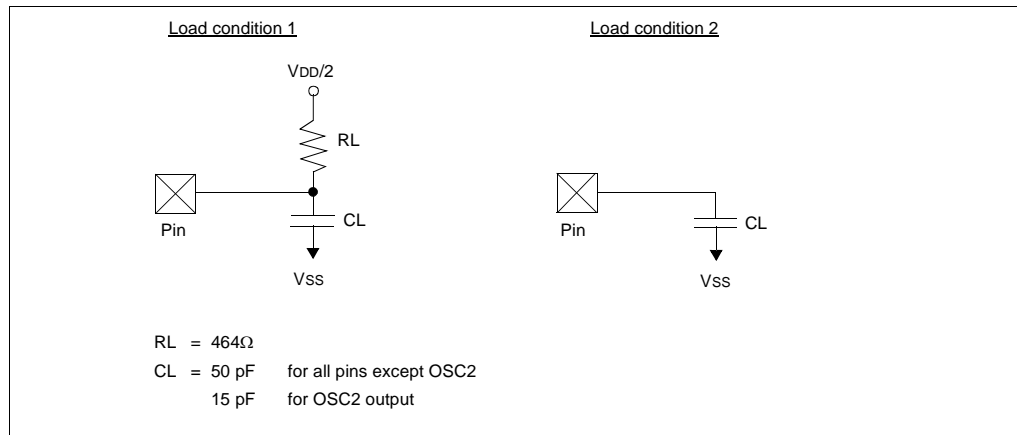
FIGURE 17-3: LOAD CONDITIONS
