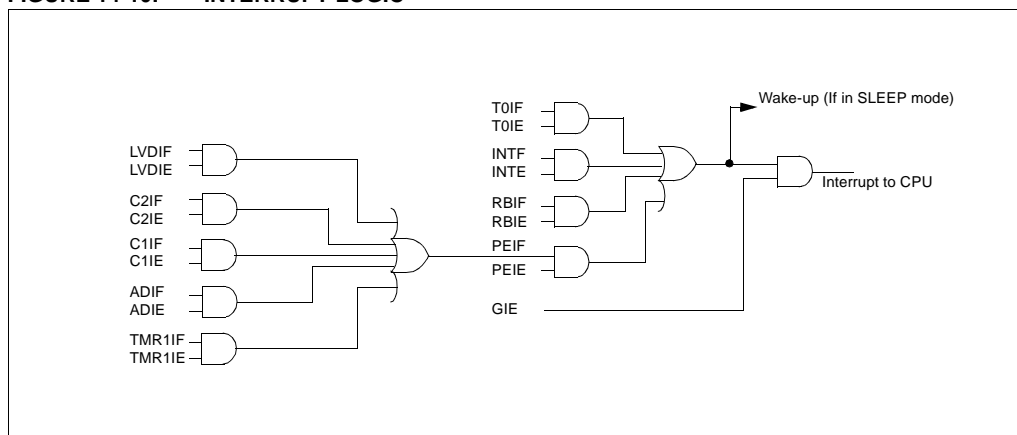
FIGURE 14-10: INTERRUPT LOGIC
