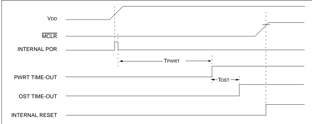
FIGURE 14-8: TIME-OUT SEQUENCE ON POWER-UP (MCLR NOT TIED TO VDD)
