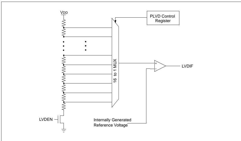
FIGURE 8-2: LOW VOLTAGE DETECT BLOCK DIAGRAM
