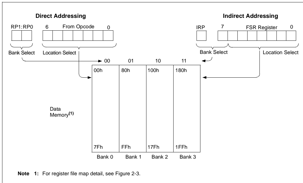
FIGURE 2-5: DIRECT/INDIRECT ADDRESSING
