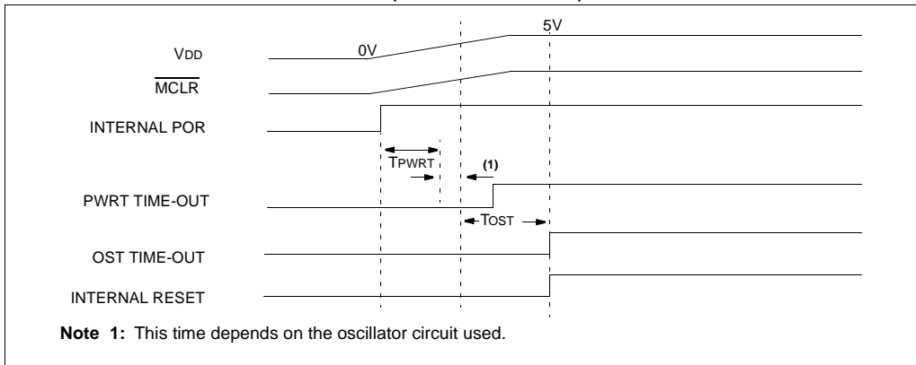
FIGURE 14-9: SLOW VDD RISE TIME (MCLR TIED TO VDD)
