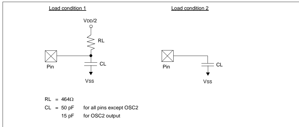
FIGURE 17-3: LOAD CONDITIONS
