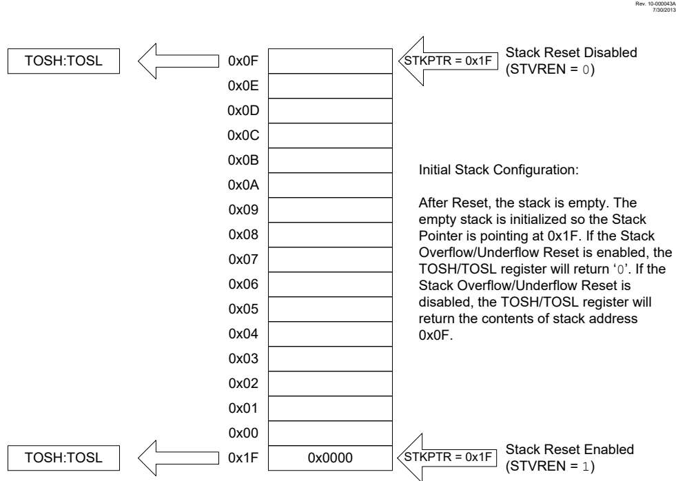
Figure 5-4. Accessing the Stack Example 1
