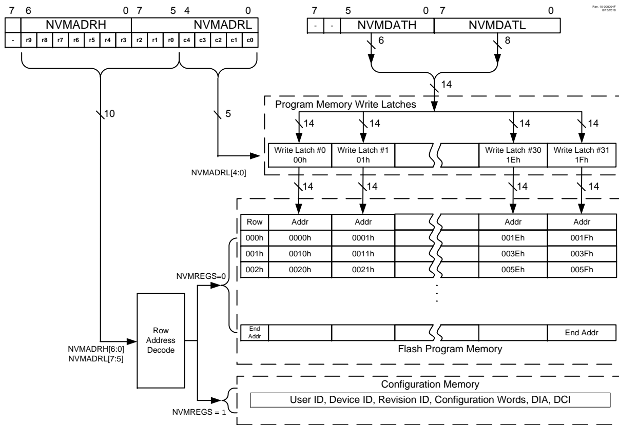
Figure 6-4. NVMREG Writes to Program Flash Memory With 32 Write Latches
