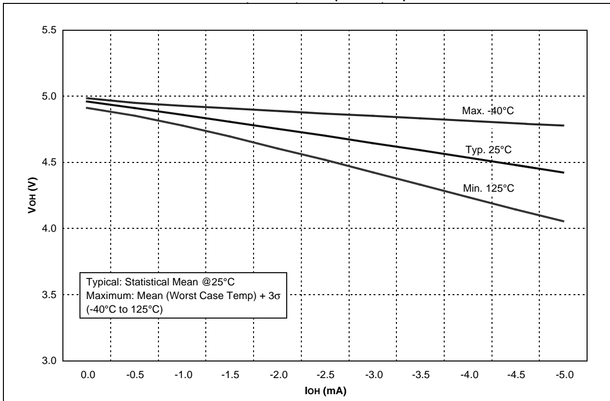
FIGURE 18-25: V_{OH} vs. I_{OH} OVER TEMPERATURE ( V_{DD} = 5.0V )
