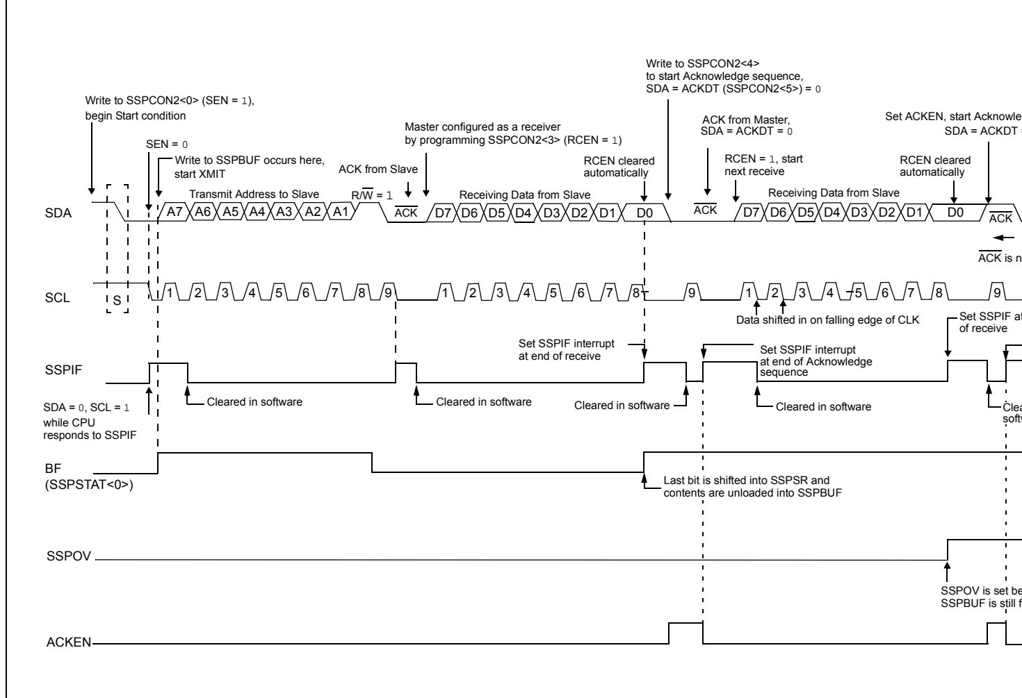
FIGURE 18-24: I 2 C MASTER MODE WAVEFORM (RECEPTION, 7-BIT ADDRESSING)
