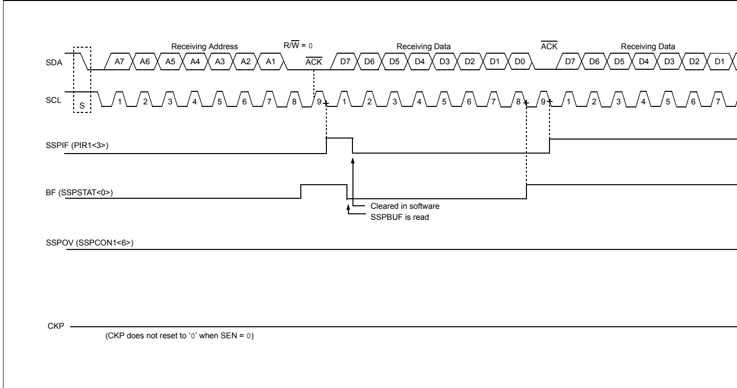
FIGURE 18-8: I 2 C SLAVE MODE TIMING WITH SEN = 0 (RECEPTION, 7-BIT ADDRESSING)
