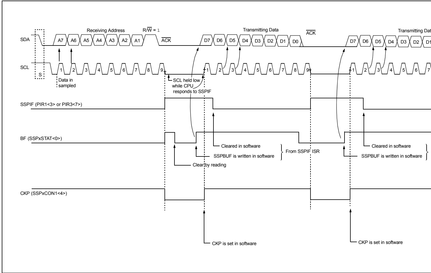
FIGURE 18-10: I 2 C SLAVE MODE TIMING (TRANSMISSION, 7-BIT ADDRESSING)
