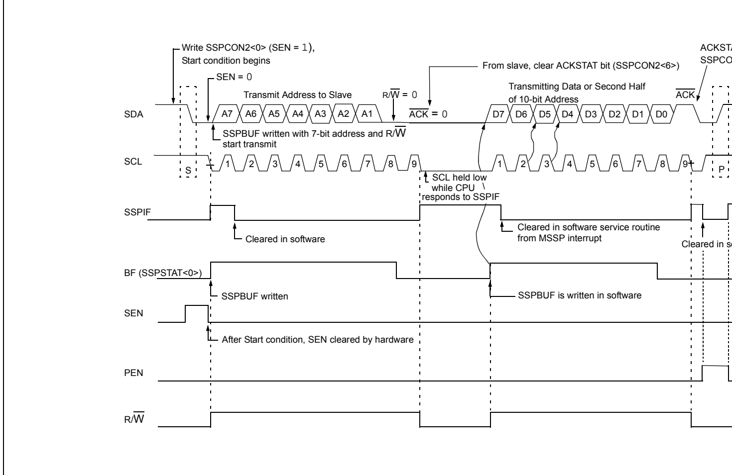
FIGURE 18-23: I 2 C MASTER MODE WAVEFORM (TRANSMISSION, 7 OR 10-BIT ADDRESSING)
