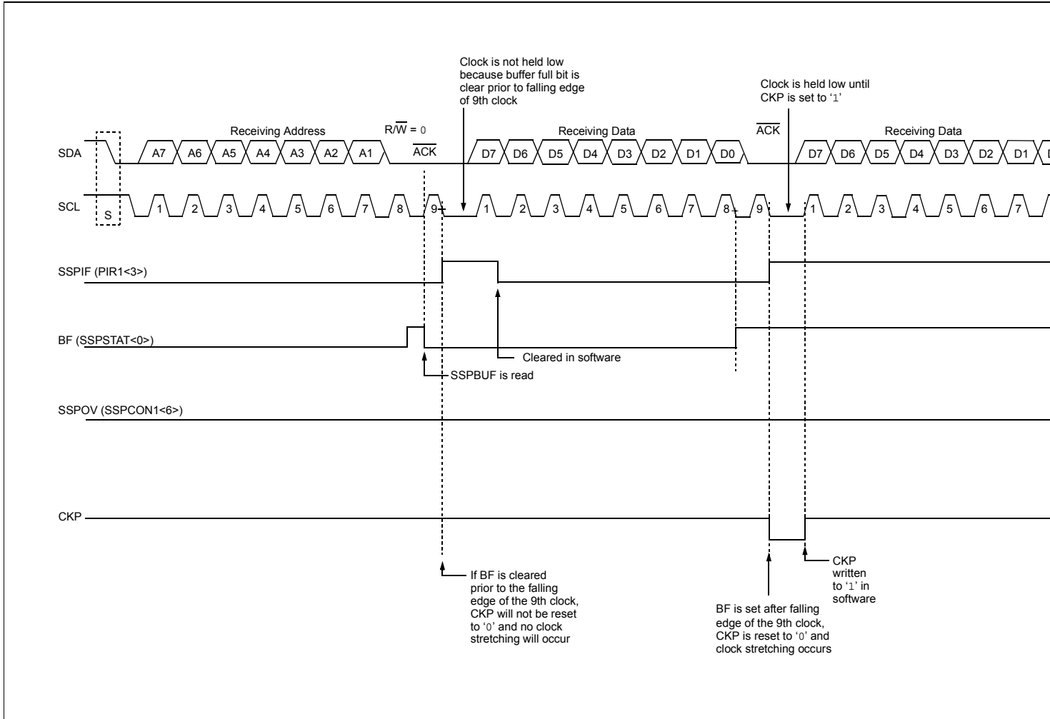
FIGURE 18-15: I 2 C SLAVE MODE TIMING WITH SEN = 1 (RECEPTION, 7-BIT ADDRESSING)
