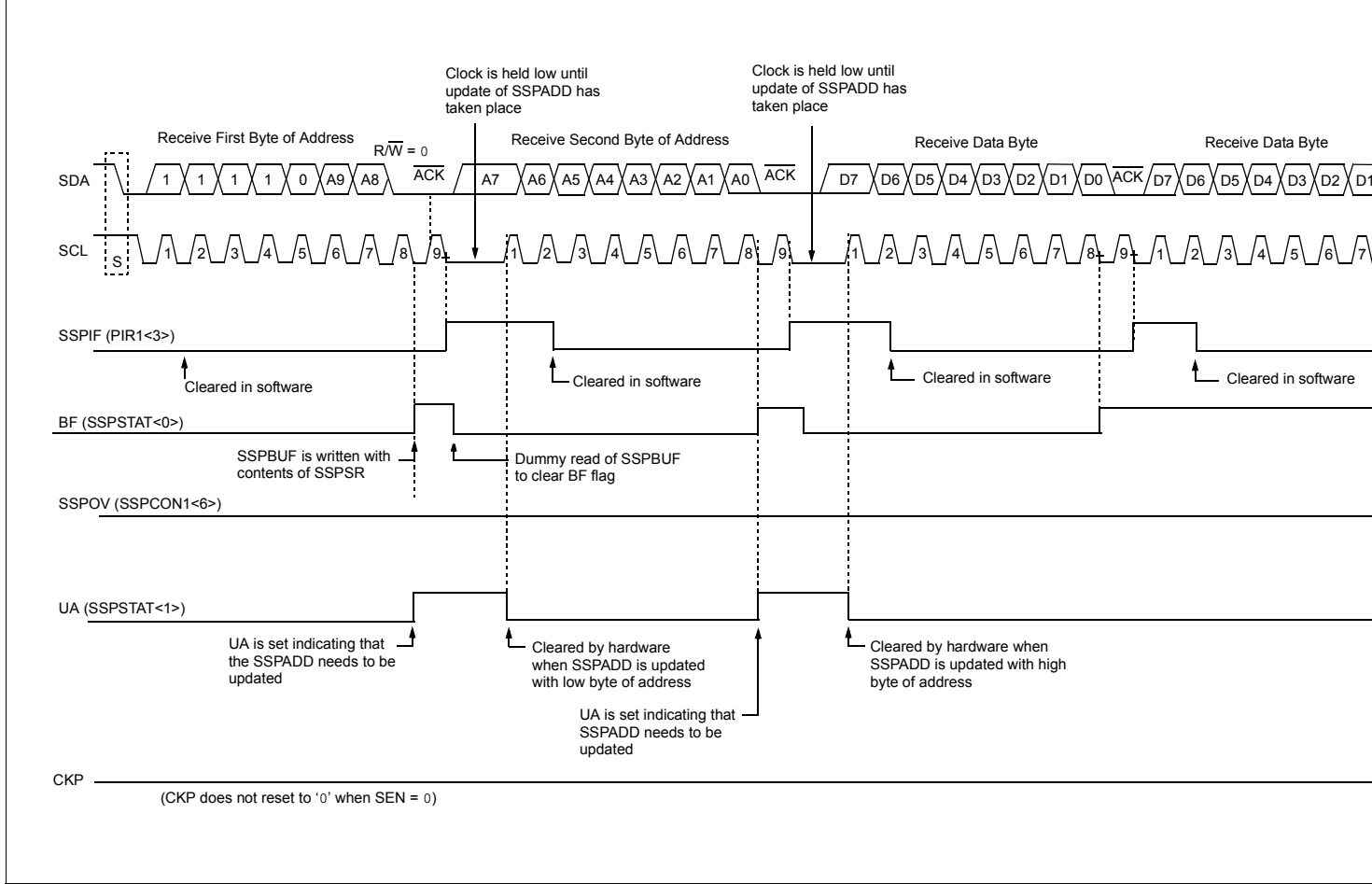
FIGURE 18-11: I 2 C SLAVE MODE TIMING WITH SEN = 0 (RECEPTION, 10-BIT ADDRESSING)
