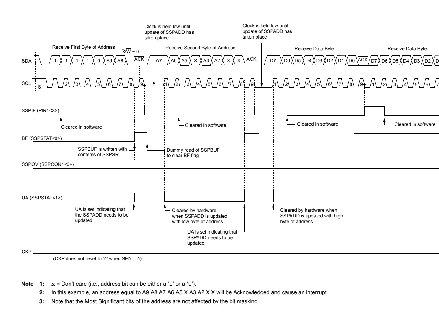
FIGURE 18-12: I 2 C SLAVE MODE TIMING WITH SEN = 0 AND ADMSK<5:1> = 01001 (RECEPTION, 10-BIT ADDRESS)
