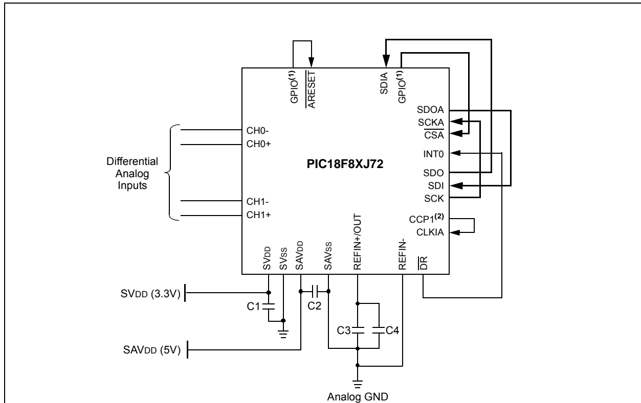
FIGURE 22-3: REQUIRED CONNECTIONS FOR AFE OPERATION
