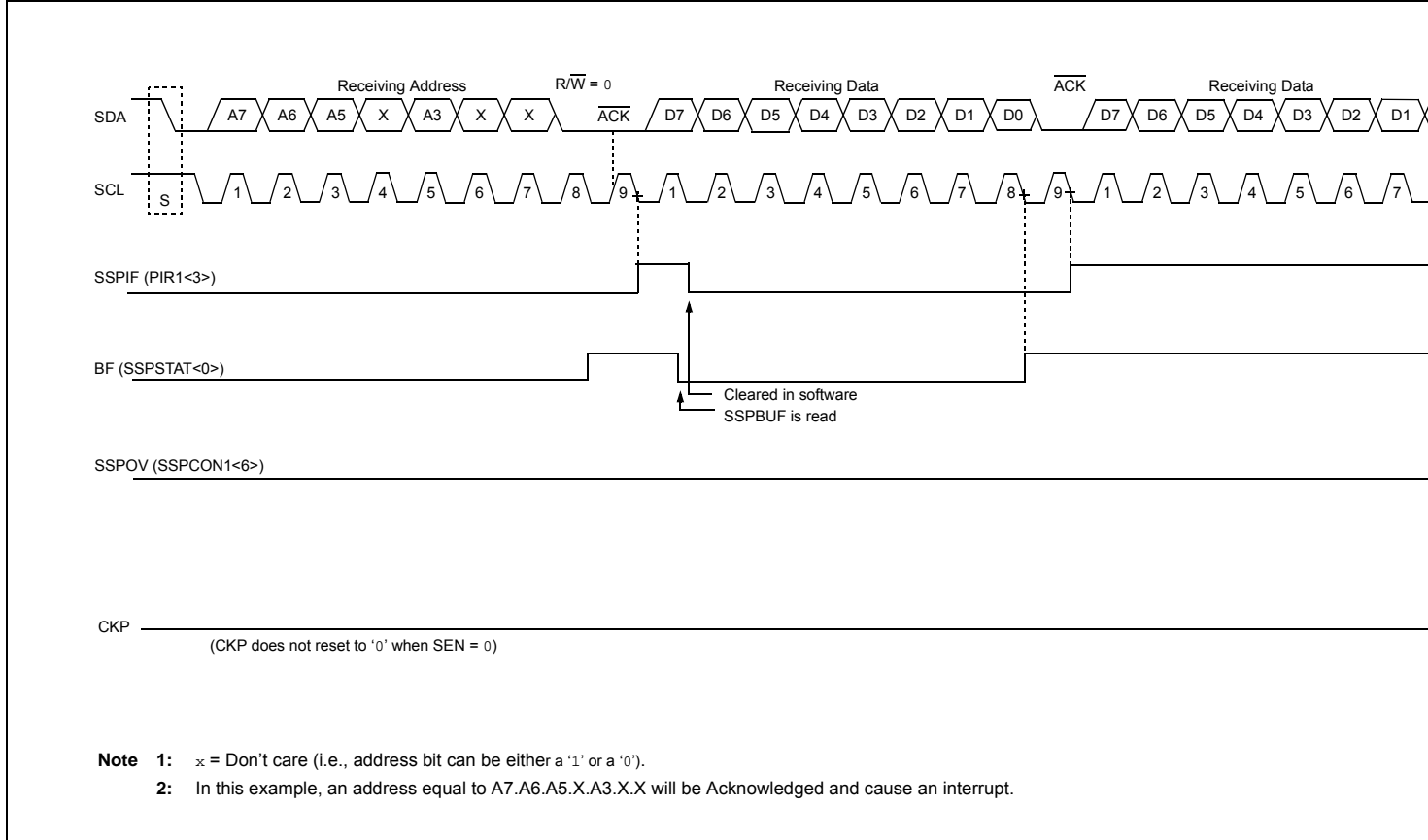
FIGURE 18-9: I 2 C SLAVE MODE TIMING WITH SEN = 0 AND ADMSK<5:1> = 01011 (RECEPTION, 7-BIT ADDRESSING)
