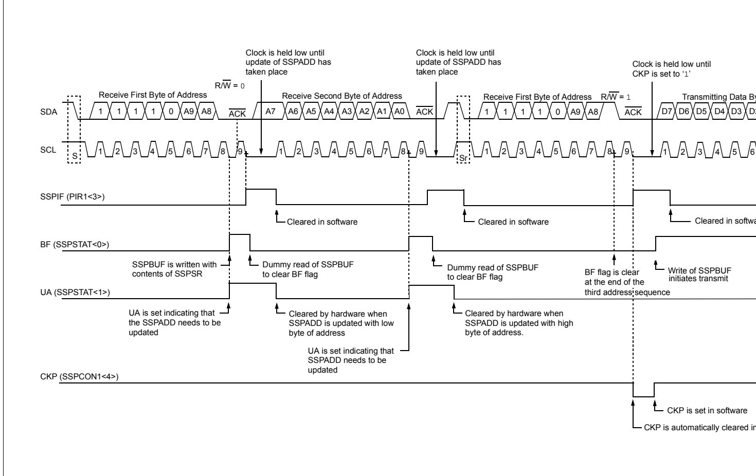
FIGURE 18-13: I 2 C SLAVE MODE TIMING (TRANSMISSION, 10-BIT ADDRESSING)
