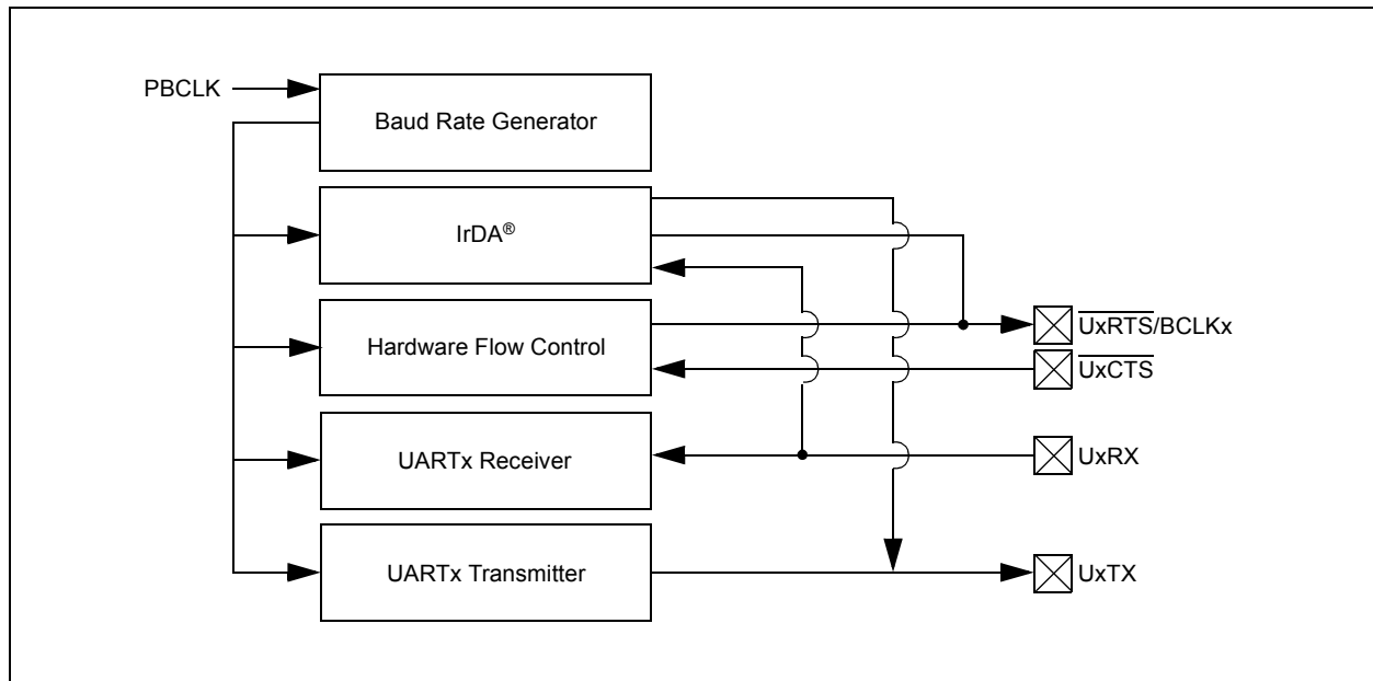
FIGURE 17-1: UARTx SIMPLIFIED BLOCK DIAGRAM
