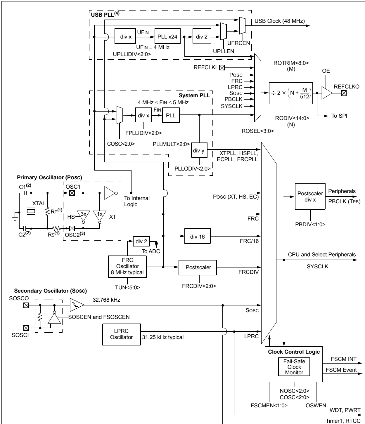
FIGURE 8-1: OSCILLATOR DIAGRAM
