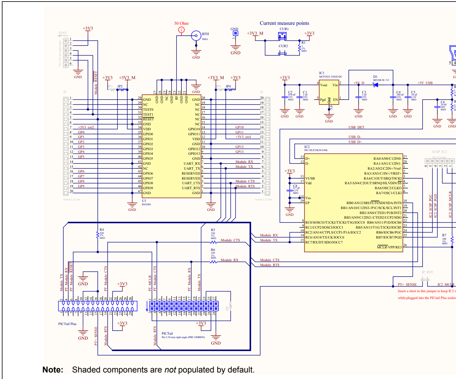
FIGURE A-1: RN2903 LoRa™ TECHNOLOGY PICtail™/PICtail PLUS DAUGHTER BOARD SCHEMATIC
