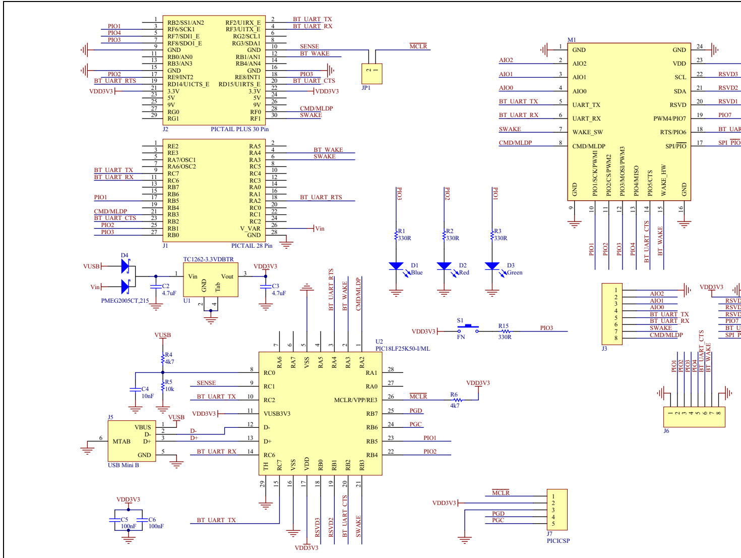
FIGURE 5-1: RN4020 TYPICAL APPLICATION SCHEMATICS
