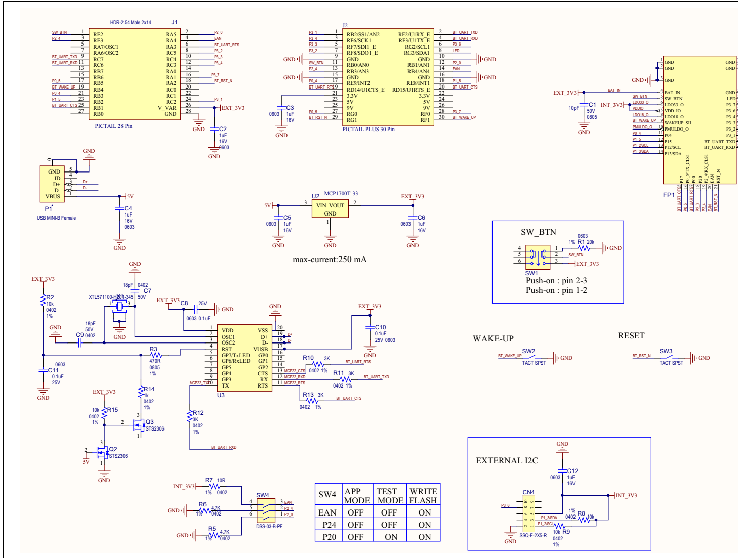
FIGURE B-1: RN4678 PICTail™/PICtail PLUS DAUGHTER BOARD SCHEMATIC
