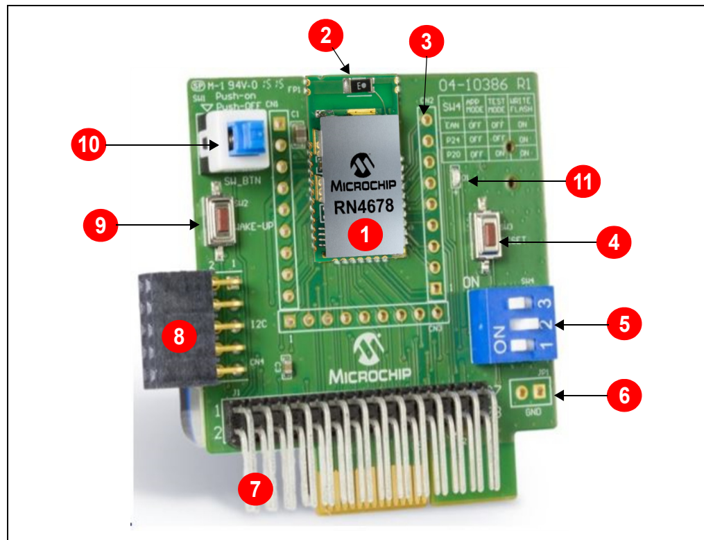
FIGURE 2-1: RN4678 PICtail™/PICtail PLUS DAUGHTER BOARD INTERFACES
