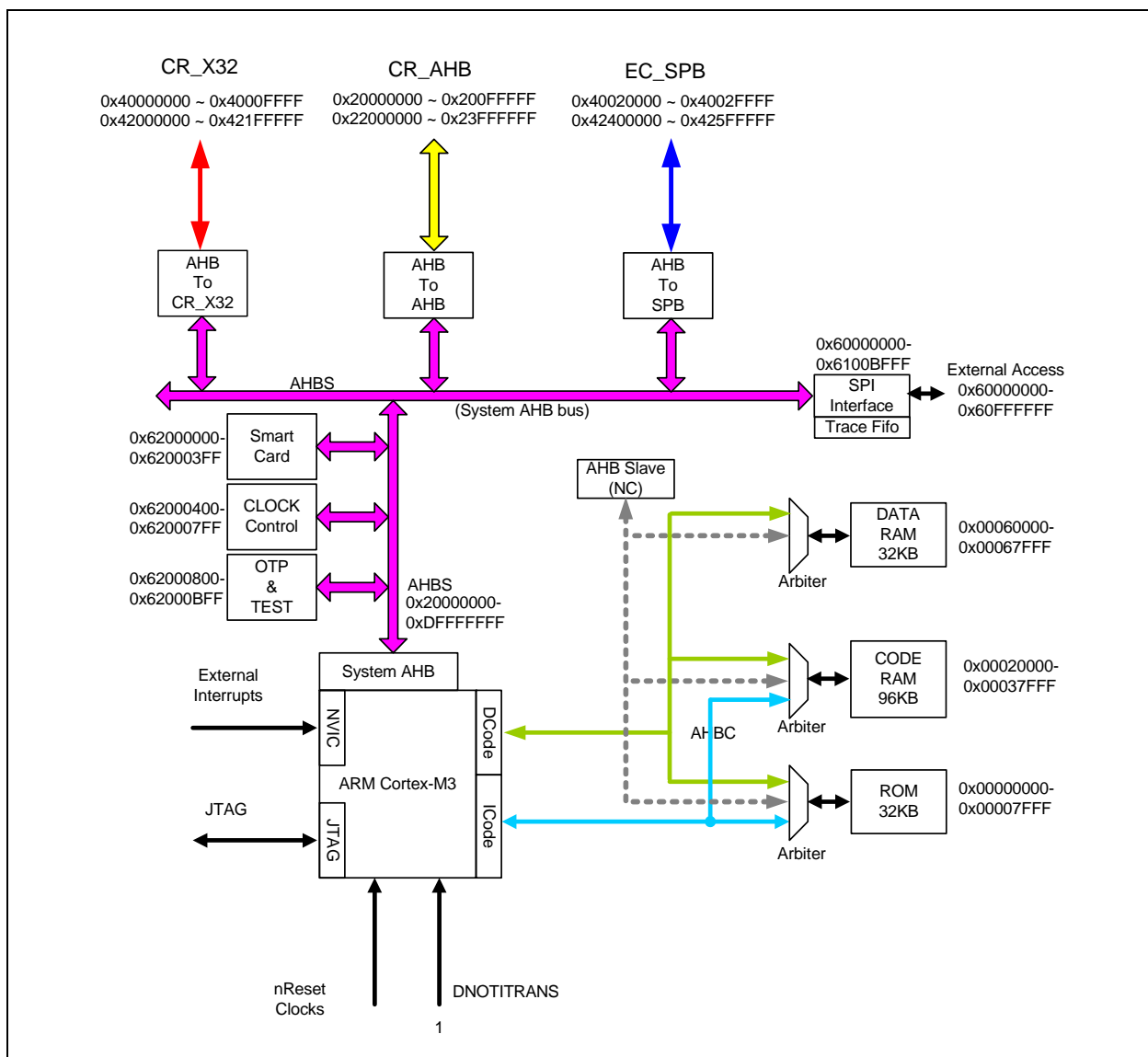
FIGURE 7-1: BUS ADDRESSES
