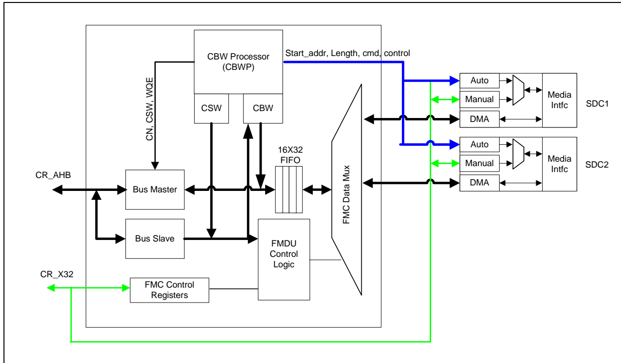
FIGURE 18-1: FLASH MEDIA DMA CONTROLLER BLOCK DIAGRAM
