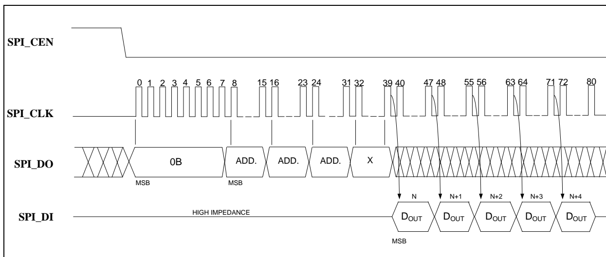
FIGURE 12-1: SPI HI-SPEED READ SEQUENCE
