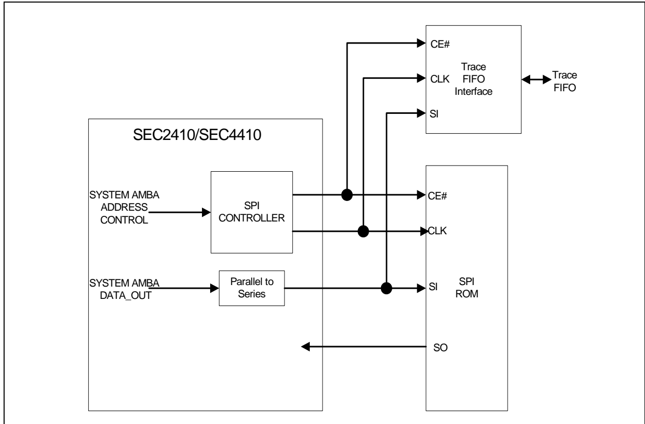
FIGURE 12-7: SPI TRACE FIFO WRITE OPERATION
