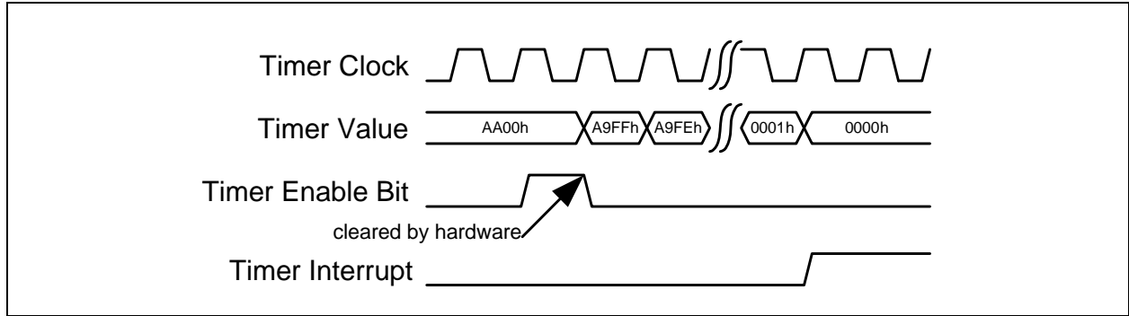
FIGURE 11-7: TIMER START BASED ON ENABLE BIT
