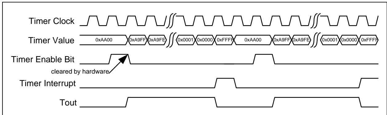
FIGURE 11-9: ONE SHOT TIMER WITH PULSE OUTPUT
