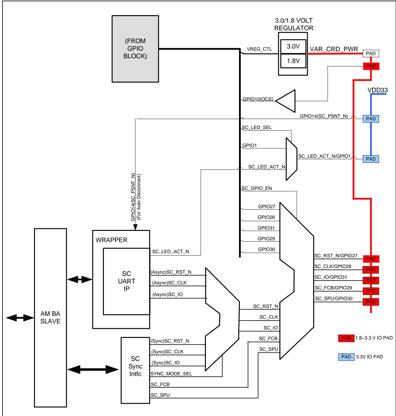
FIGURE 13-13: SMARTCARD MUXING
