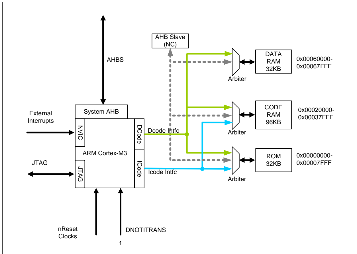
FIGURE 4-1: ARM Block Diagram
