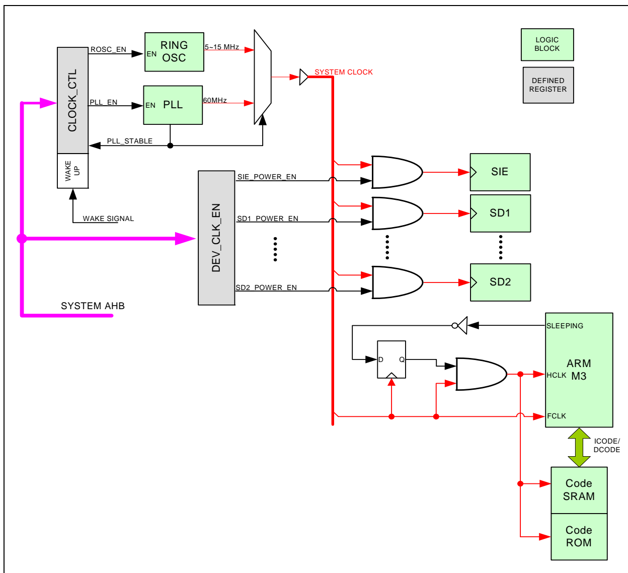
FIGURE 23-1: CLOCK CONTROL BLOCK DIAGRAM
