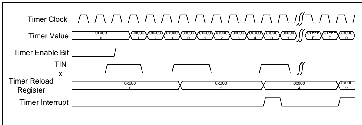
FIGURE 11-11: PULSE PERIOD MEASUREMENT
