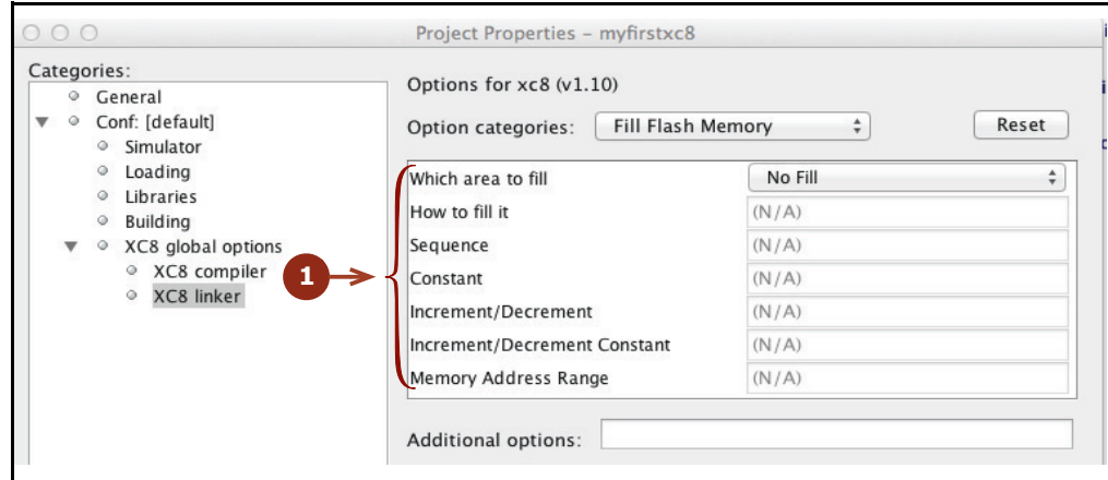
FIGURE 4-11: FILL FLASH MEMORY OPTIONS
