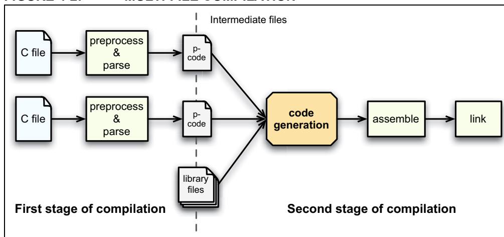
FIGURE 4-2: MULTI-FILE COMPILATION
