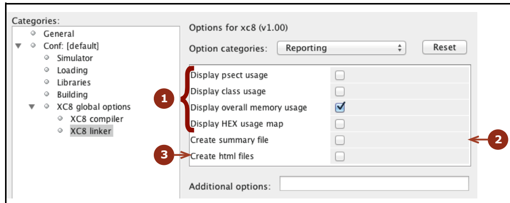
FIGURE 4-13: REPORTING OPTIONS
