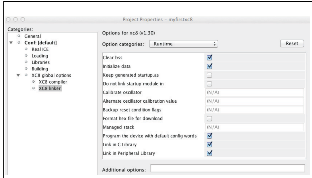
FIGURE 4-9: RUNTIME OPTIONS
