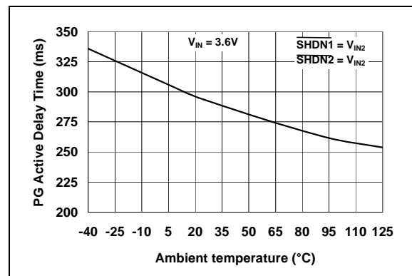
FIGURE 2-30: PG Active Delay Time-out vs. Ambient Temperature.
