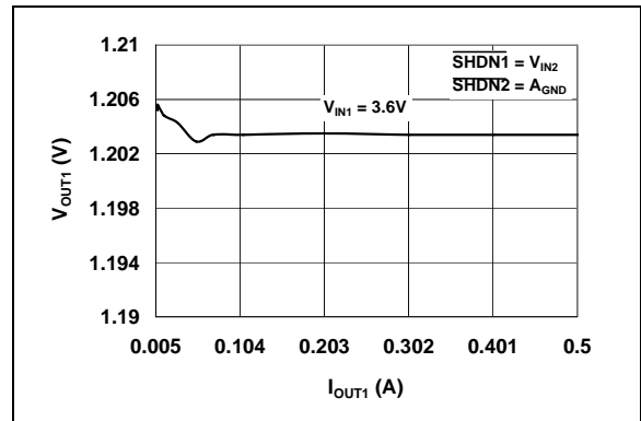
FIGURE 2-11: V_{OUT1} vs. I_{OUT1} ( V_{OUT1} = 1.2\text{V} ).
