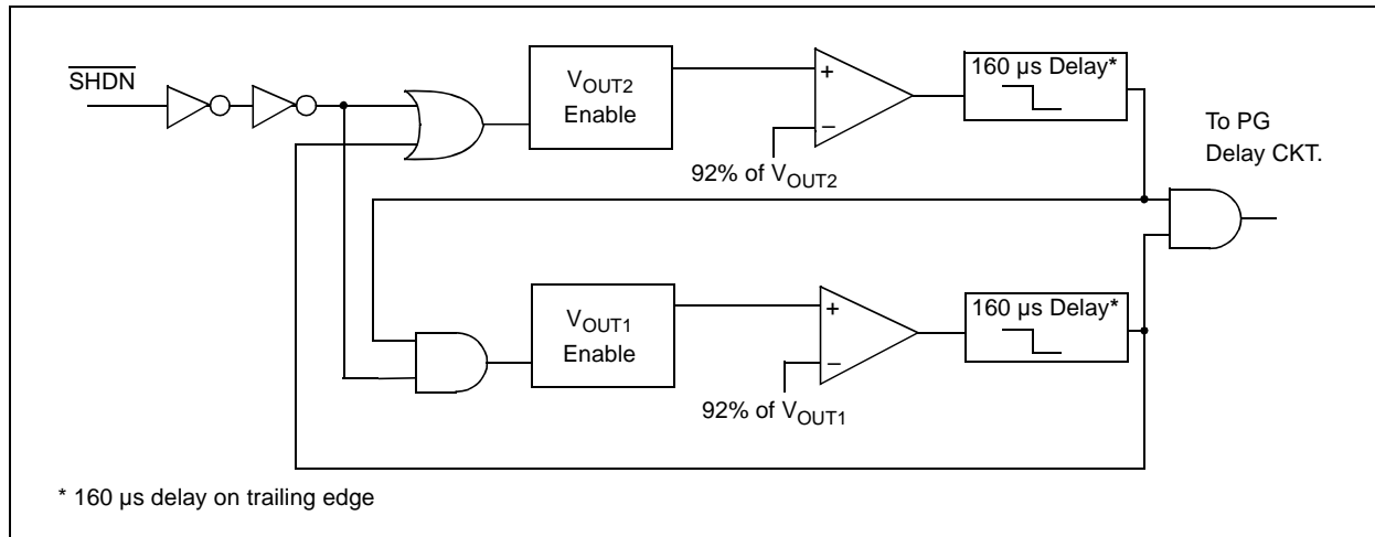
FIGURE 4-2: TC1304 Sequencing Circuit.
