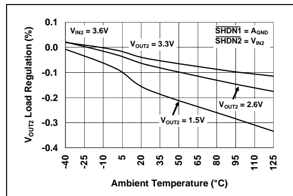
FIGURE 2-29: V_{OUT2} Load Regulation vs. Ambient Temperature.
