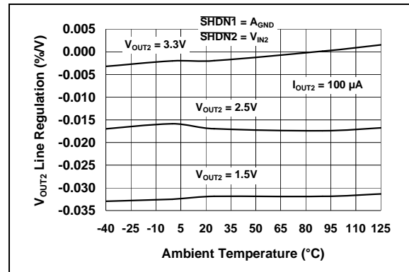
FIGURE 2-28: V_{OUT2} Line Regulation vs. Ambient Temperature.
