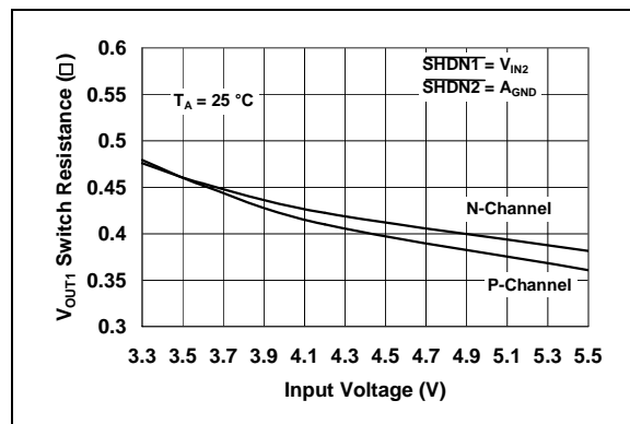
FIGURE 2-17: V_{OUT1} Switch Resistance vs. Input Voltage.
