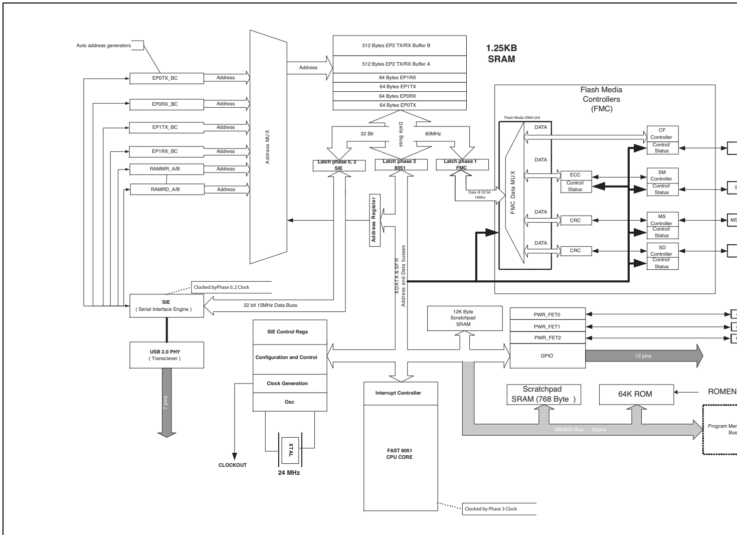
FIGURE 3-1: USB2227/USB2228 BLOCK DIAGRAM
