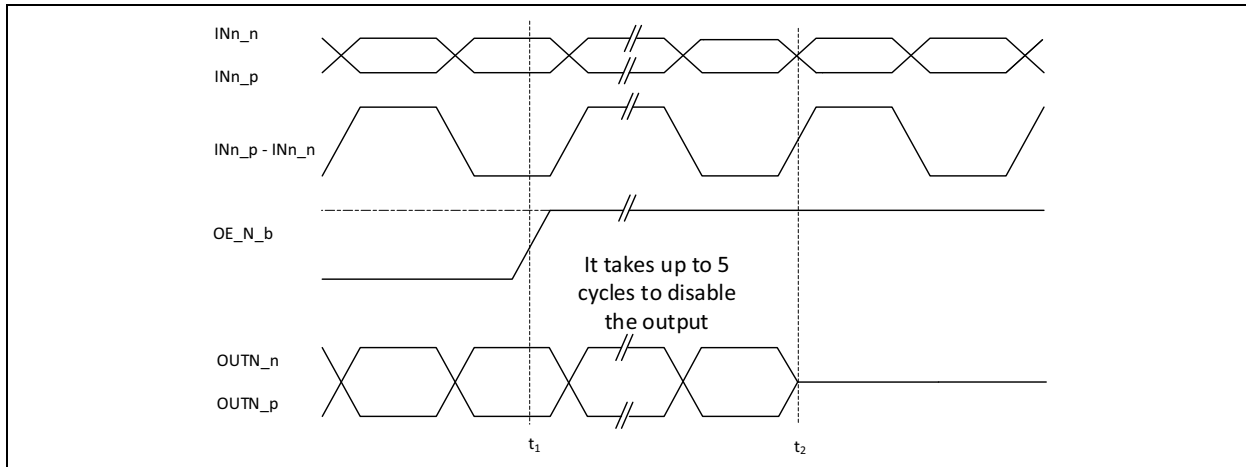
FIGURE 2-12: Output Disable.
