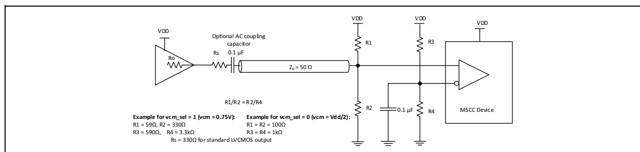
FIGURE 2-1: Input Driven by a Single-Ended Output for vcm_sel = 0 and 1.
