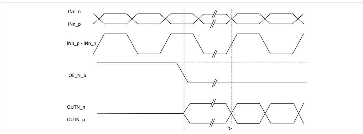
FIGURE 2-13: Output Enable.
