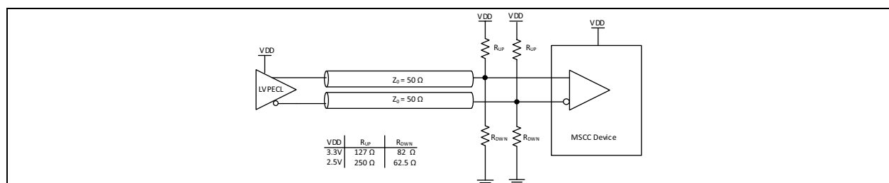
FIGURE 2-2: Input Driven by DC-Coupled LVPECL Output for vcm_sel = 0.
