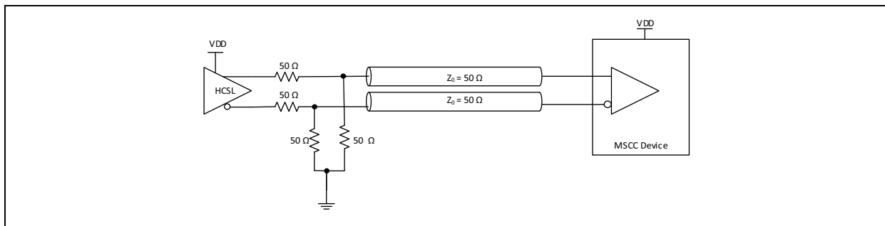
FIGURE 2-5: Input Driven by HCSSL Output for vcm\_sel = 1 .
