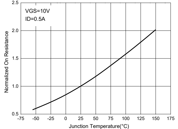
Fig.6-NormalizedOnResistanceCharacteristics
