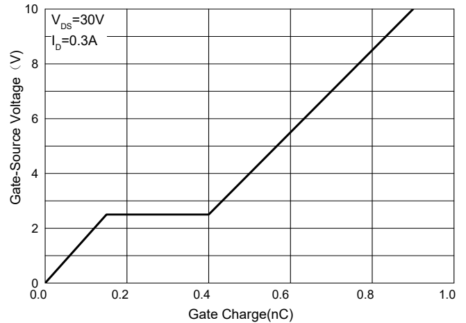
Fig.6 - Gate Charge
