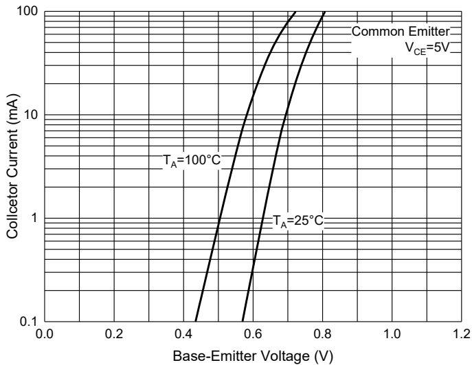
Fig. 5 - Base-Emmitter Voltage Characteristics
