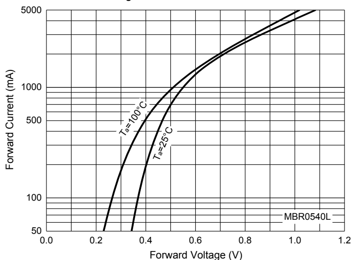
Fig. 3 - Forward Characteristics
