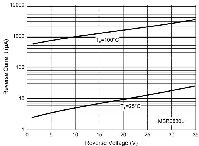
Fig. 5 - Reverse Characteristics
