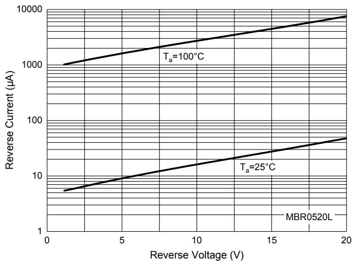
Fig. 4 - Reverse Characteristics
