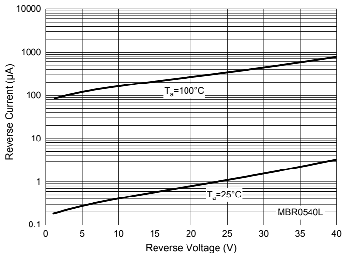
Fig. 6 - Reverse Characteristics
