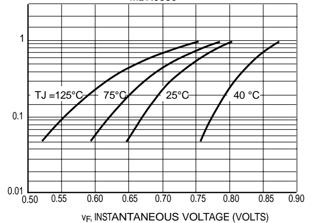
Figure 6 Typical Forward Characteristics MBR0580
