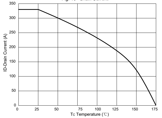
Fig. 10 - Drain Current
