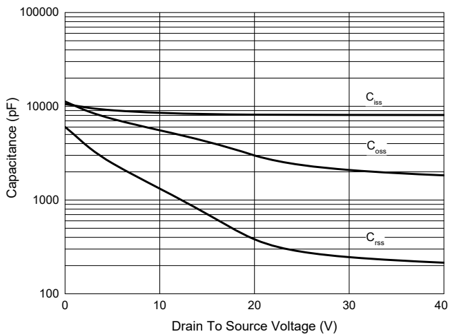
Fig. 5 - Capacitance Characteristics
