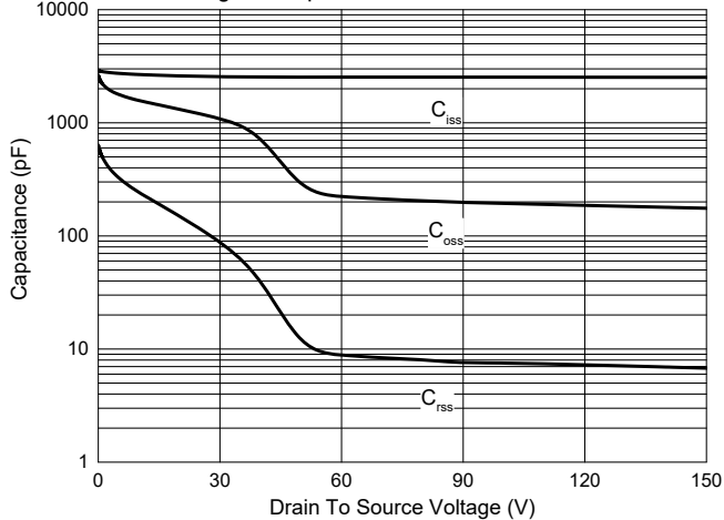
Fig. 5 - Capacitance Characteristics
