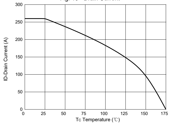
Fig. 10 - Drain Current
