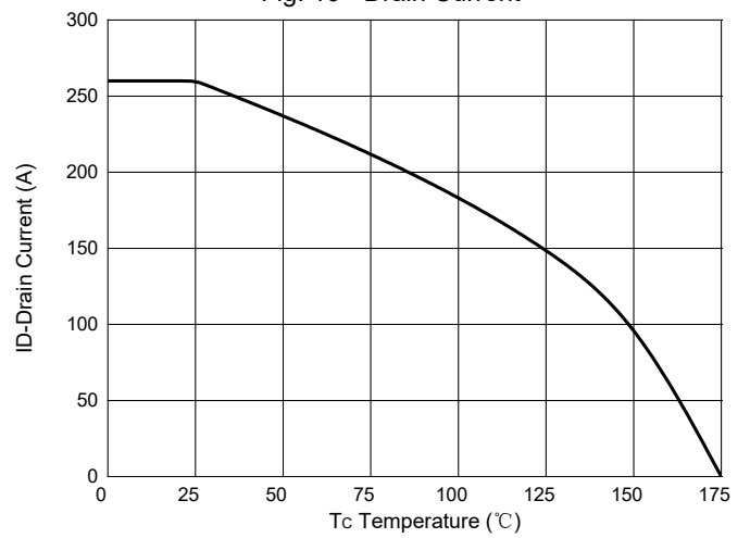
Fig. 10 - Drain Current
