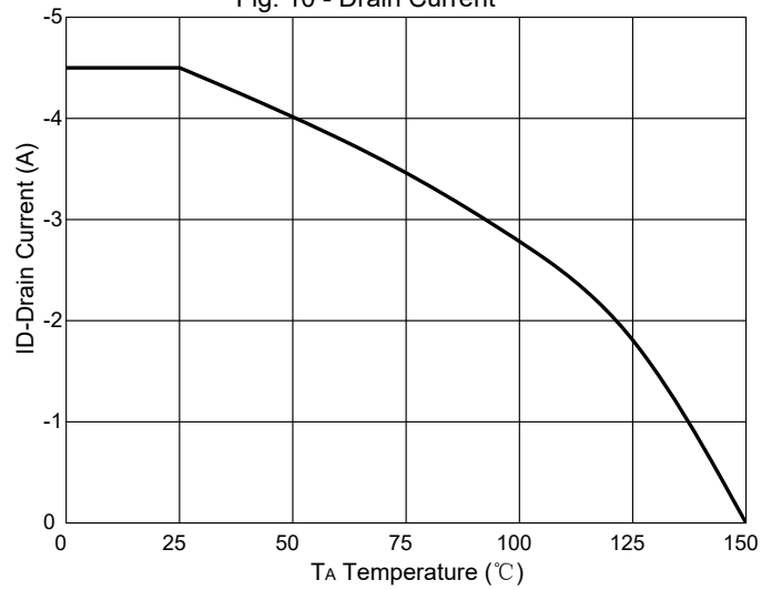
Fig. 10 - Drain Current
