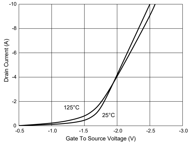
Fig. 9 - Transfer Characteristics
