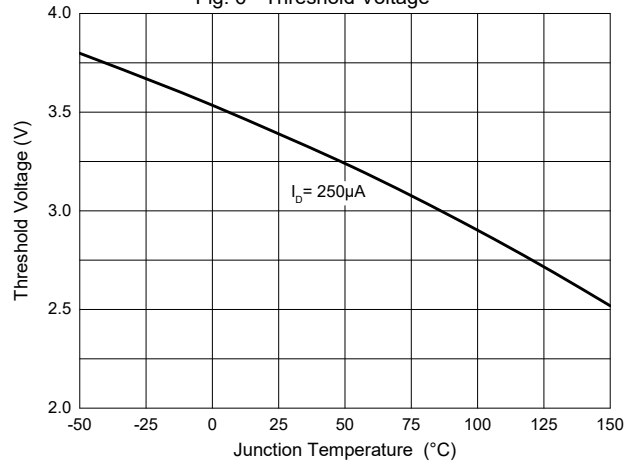
Fig. 6 - Threshold Voltage
