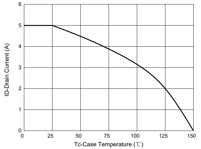
Fig. 10 - Current dissipation
