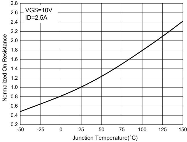
Fig.9-NormalizedOnResistanceCharacteristics
