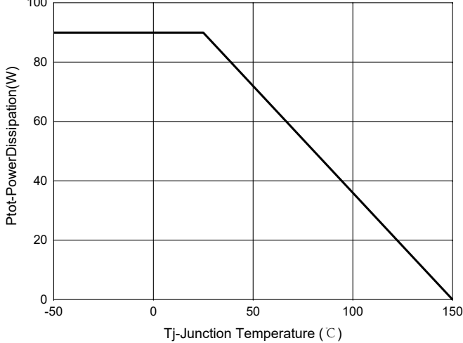
Fig.11-PowerDissipation
