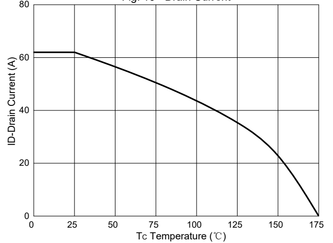
Fig. 10 - Drain Current
